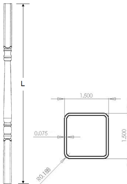
FIGURE 2 – VINYL SPINDLE
