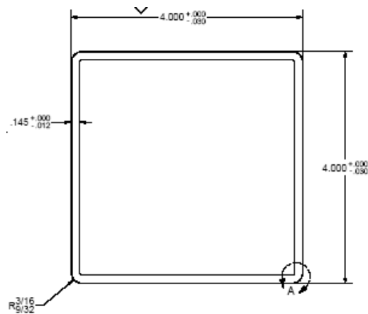
4" Square STD Post
