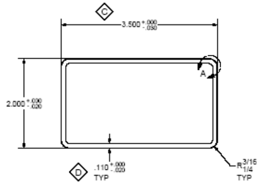
2" x 3.5" STD Rail
