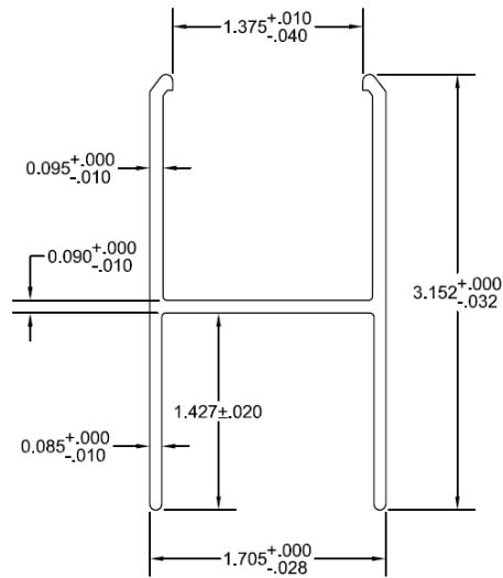
FIGURE 2 – ALUMINUM "H" CHANNEL INSERT
