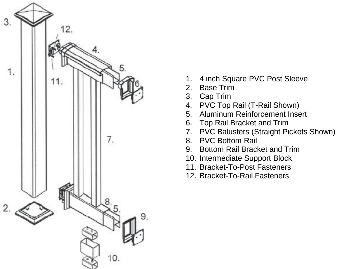
Figure 2 - Typical Rail Assembly
