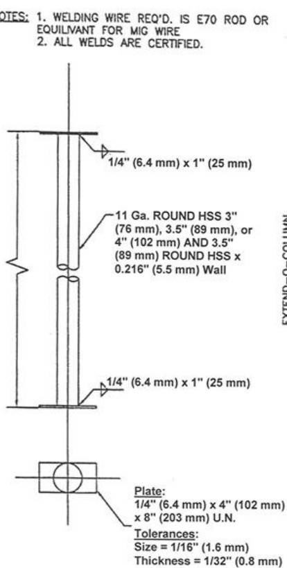
Figure 1 - Fixed Length Column
