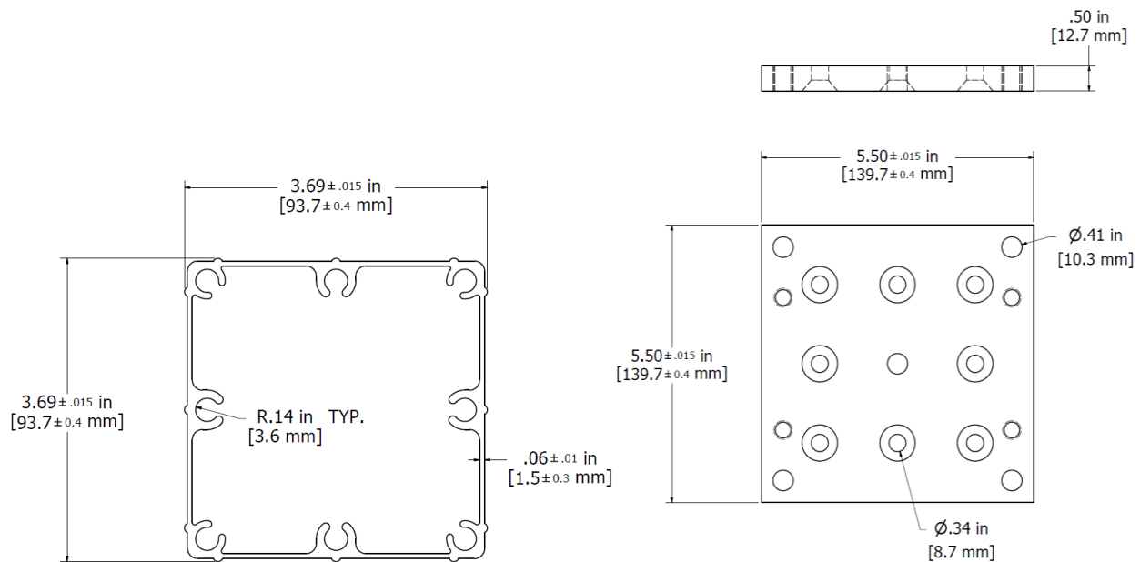
Figure 4 - 4 x 4 Post Mount Aluminum Insert
