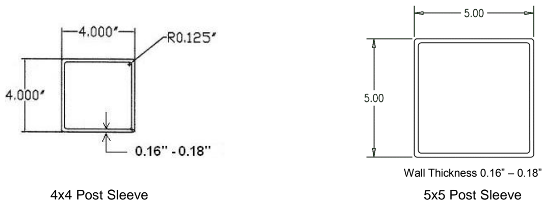
Figure 3 – TAM-RAIL® Post Sleeve Cross Sections
