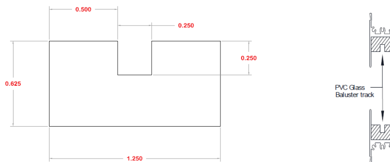
Figure 18 – Liberty Support Channel for Glass Balusters
