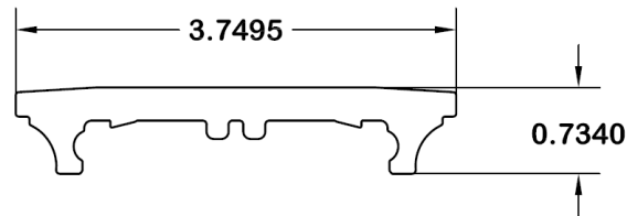
Figure 26 – Rockport Top Rail Cap
