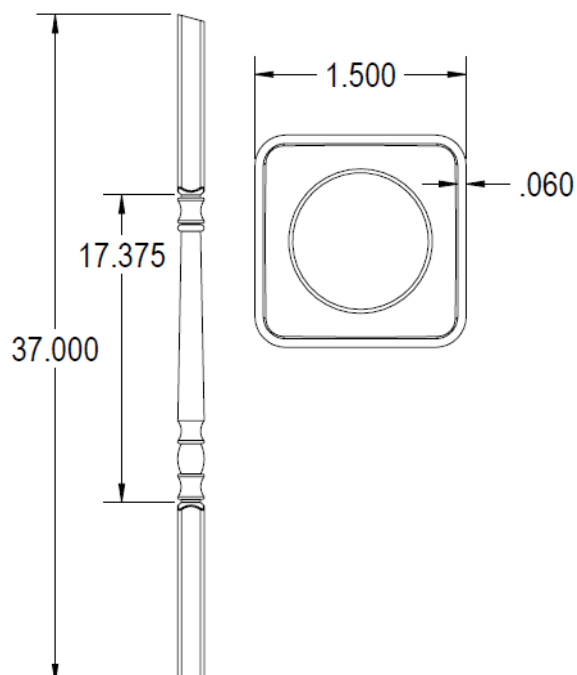
Figure 17 – Excel PVC Spindle and Turned (T)
