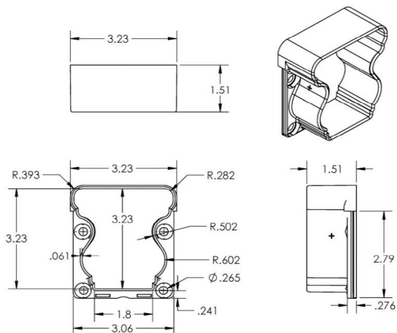
Figure 25 – 3000 Series Newport Rail Top Rail Mounting Bracket
