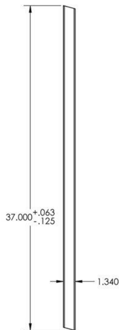
Figure 14 – Model PVC Baluster
