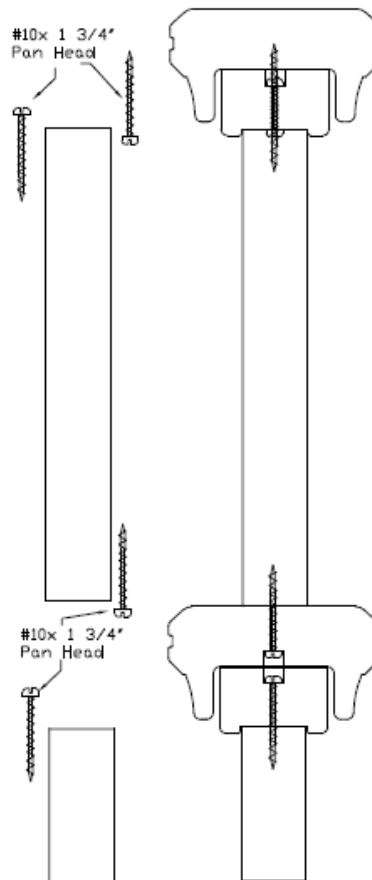
Figure 22 – Square WPC Baluster Assembly
