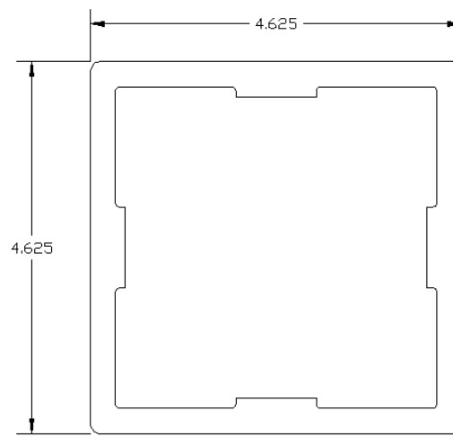
Figure 4 – Post Sleeve
