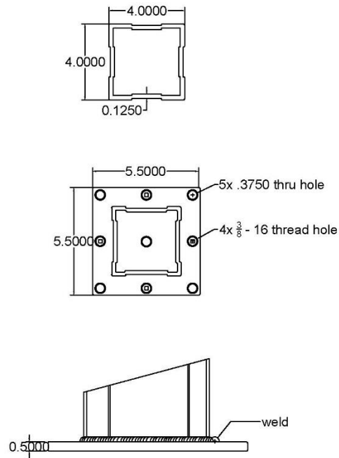
FIGURE 21 - 4 IN. WELDED POST
