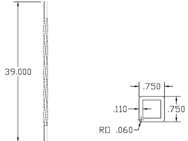
FIGURE 16 - HAMMERED AND TWISTED BALUSTER
