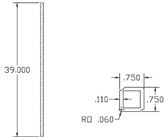
FIGURE 14 - HAMMERED BALUSTER
