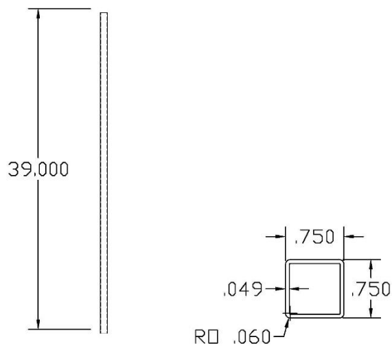
FIGURE 11 - SQUARE BALUSTER
