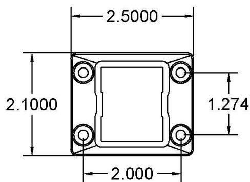
FIGURE 9 - KEYSTONE, AMERICAN, AND ARABIAN BOTTOM RAIL BRACKETS
