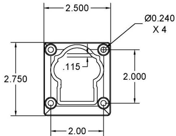
FIGURE 7 - ARABIAN TOP RAIL BRACKET
