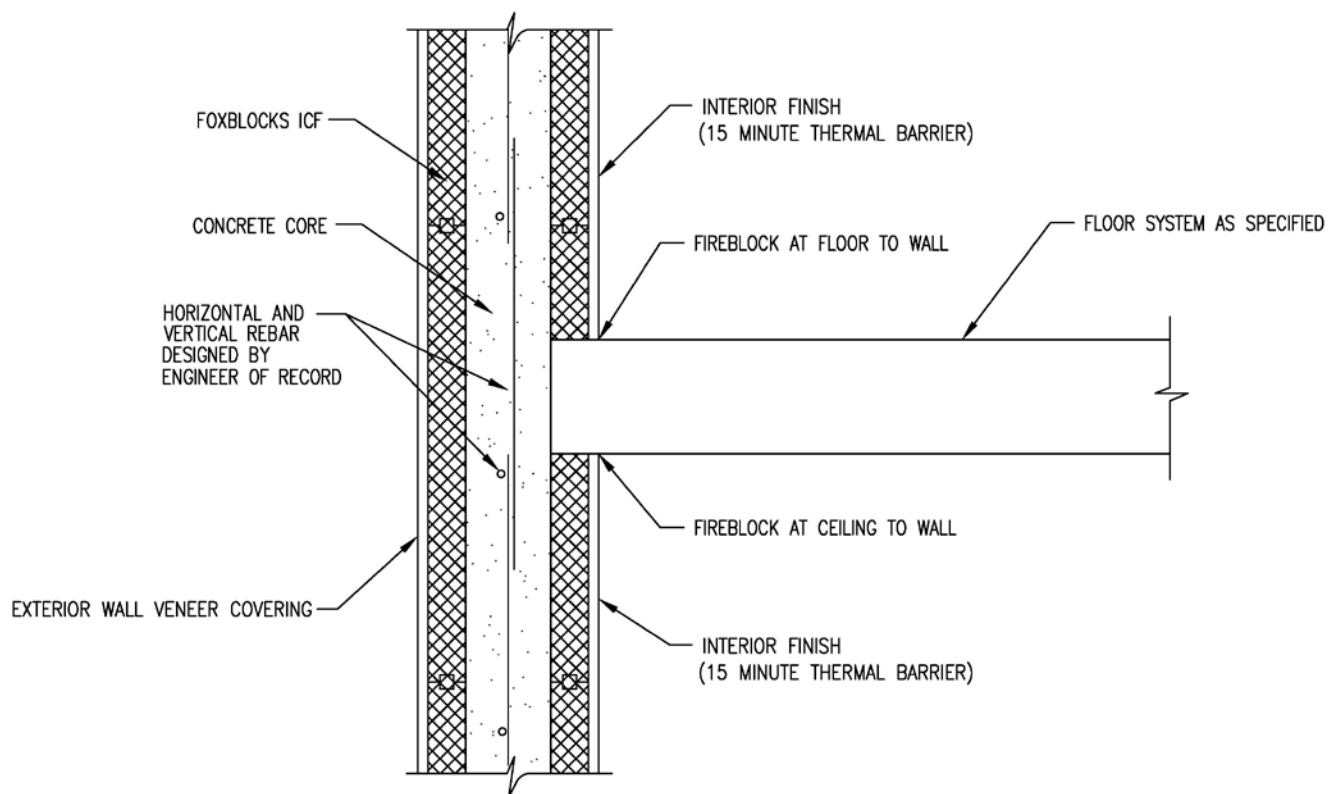
Figure 3 – TYPICAL WALL-TO-FLOOR INTERSECTION FOR TYPES I, II, III, AND IV CONSTRUCTION
