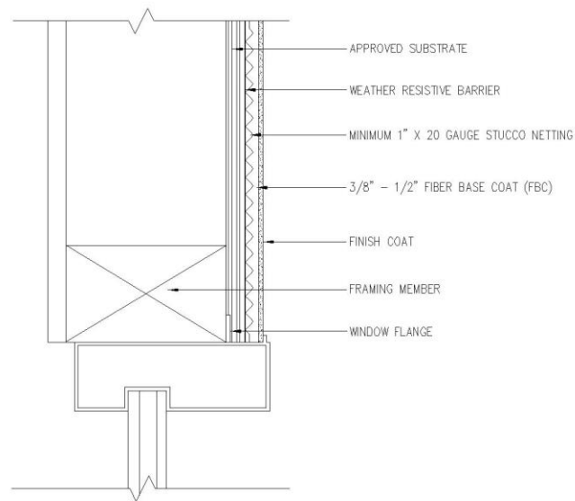
TYPICAL WINDOW – SOLID SUBSTRATE
