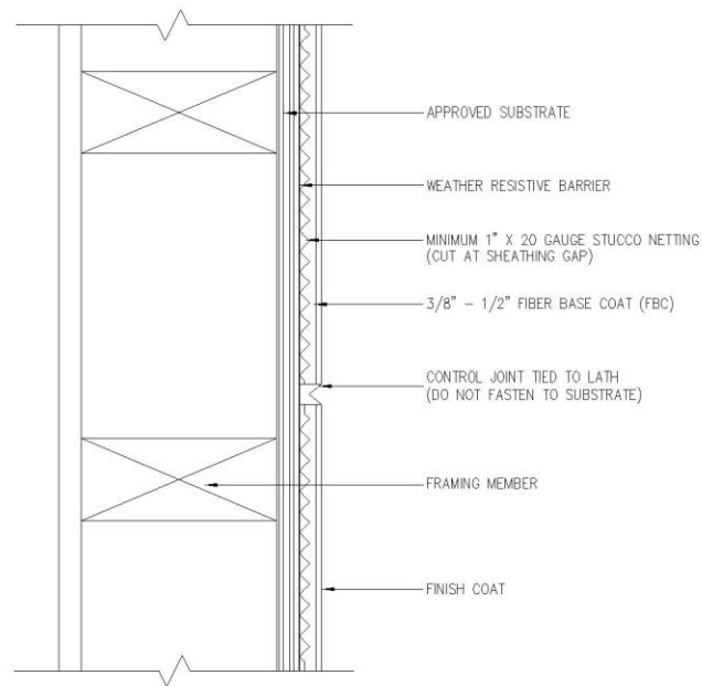
CONTROL JOINT
