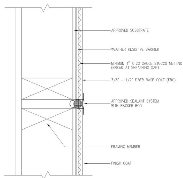
EXPANSION JOINT
