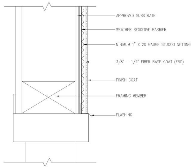
TYPICAL DOOR – SOLID SUBSTRATE
