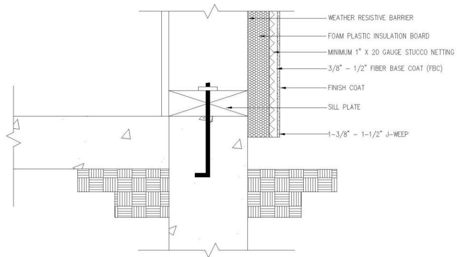
WEEP SCREED — FOAM SUBSTRATE (1)
