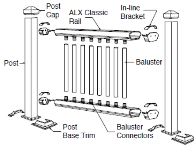
Figure 6 – Exploded View of Typical Installation
