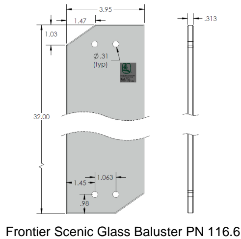
Figure 2 Continued – Balusters
