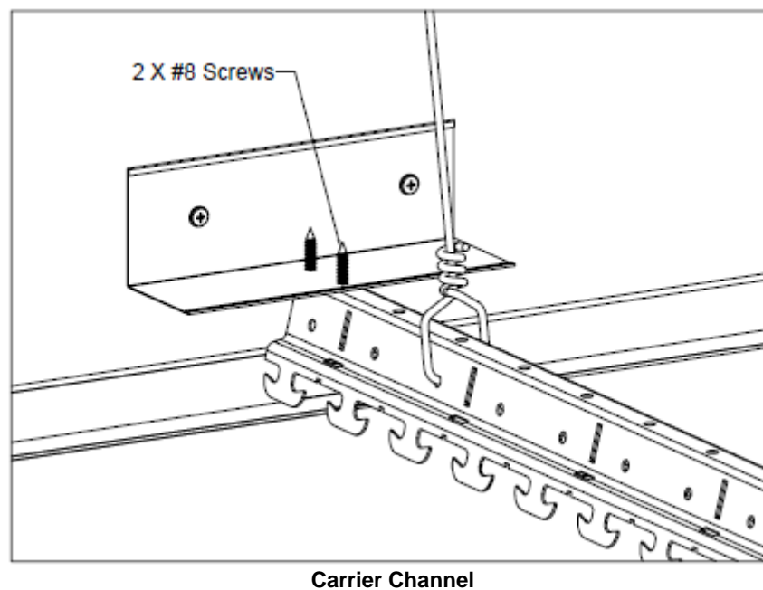
Figure- 10 Seismic Installation Attached Wall
